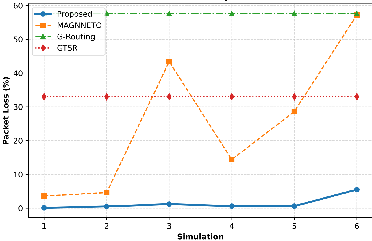
Packet Loss Comparison
